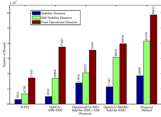
Fig. 2. Comparative Stability Analysis of Existing and Proposed Methods Across Rounds.
